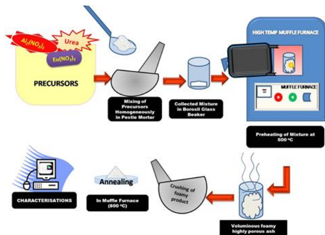
Fig. 1. Schematic illustrations of the synthesis process of \text{Al}_2\text{O}_3 : \text{Eu}^{3+} nano-powder using combustion method.
