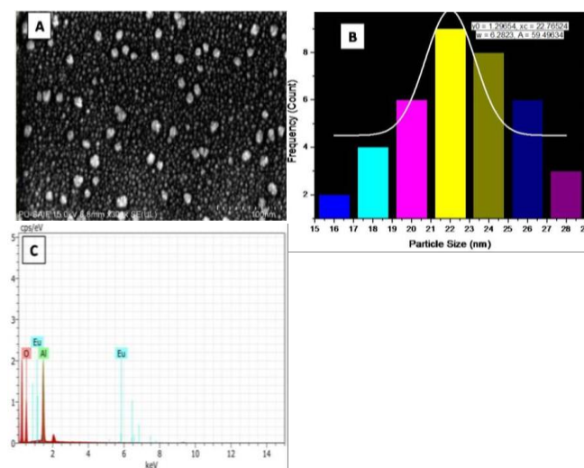
Fig. 3. (a) FE-SEM Micrograph, (b) their particle size distribution and (c) SEM-EDXA of \text{Al}_2\text{O}_3\text{:Eu}^{3+} nanocrystals showing the elemental composition.
