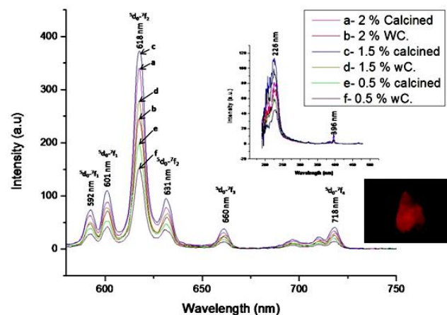
Fig. 4. Photoluminescence spectra of \text{Al}_2\text{O}_3\text{:Eu}^{3+} nanopowder showing emissions at wavelength 618 nm, 592 nm, 601 nm and 631 nm when excited with 226 nm wavelength. Inset graph is the PLE excitation spectrum showing intense band at 226 nm and a weak band at 396 nm.
