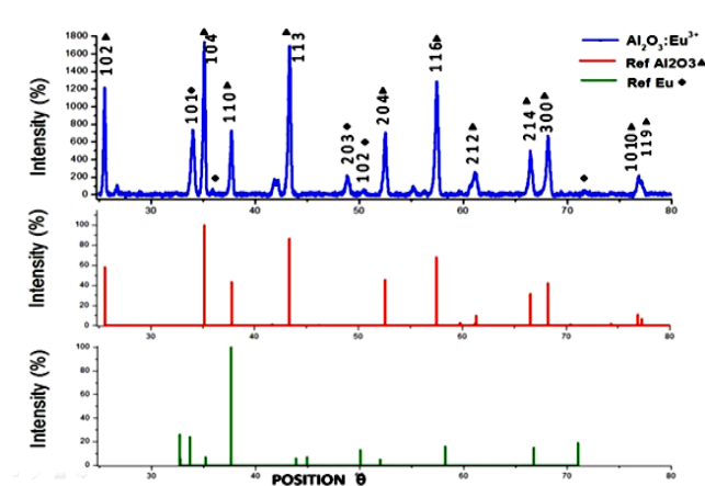
Fig. 2. XRD patterns of prepared \alpha\text{-Al}_2\text{O}_3 : \text{Eu}^{3+} (1.5mole %) is in good agreement with the standard pattern (reference code 01-074-1081), while few minor peaks are contributed by Europium.
